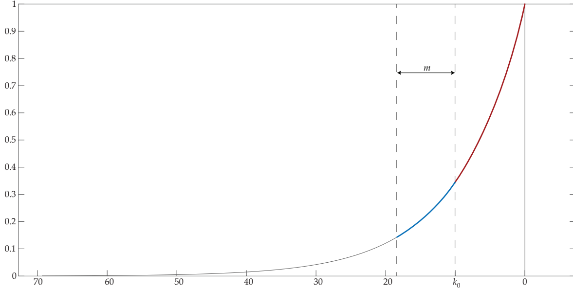
Figure 2: Moving Average coefficients of (1 - 0.9F)(1 - 0.05F)X_t = \varepsilon_t
