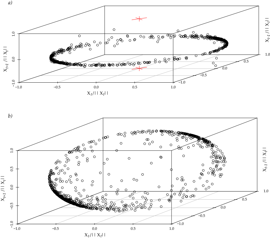
Figure 1: Moving Average coefficients of (1 - 0.9F)(1 - 0.05F)X_t = \varepsilon_t
