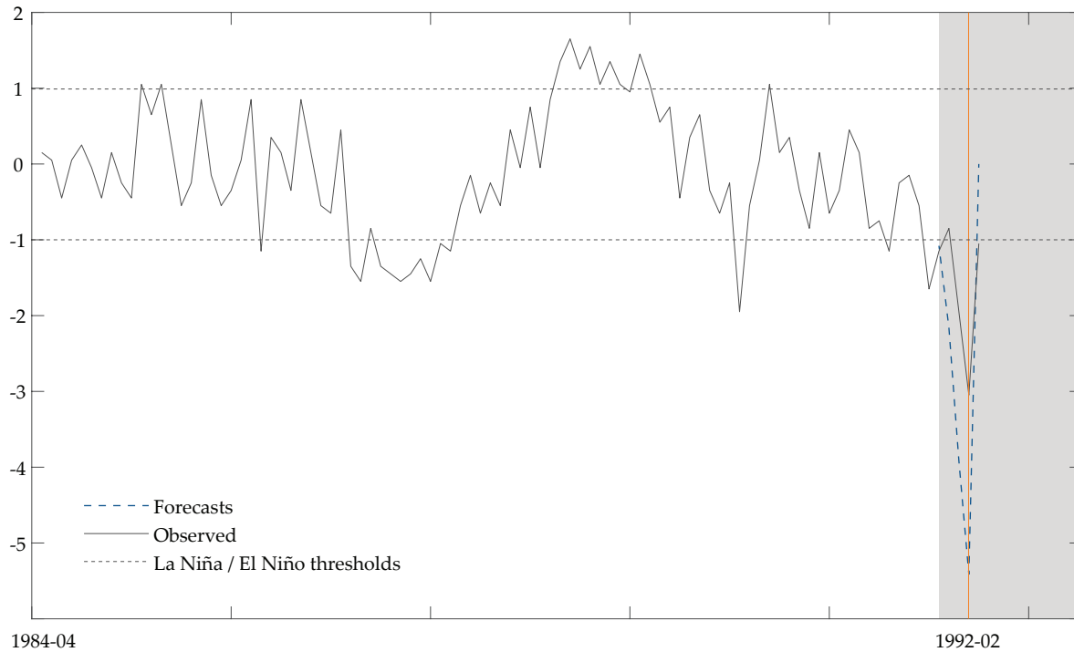
Figure 4: La Niña reversal forecast
